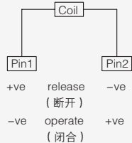
单线圈 Single coil
