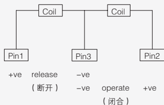
双线圈 Double coil
