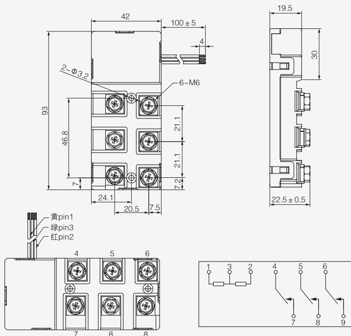
双线圈 Double coil
