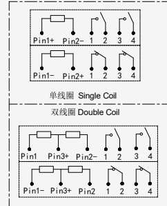
反极性Reverse polarity
