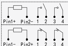
单线圈 Single coil
