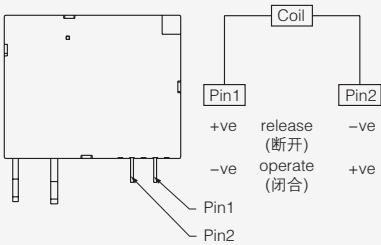
单线圈 Single Coil
