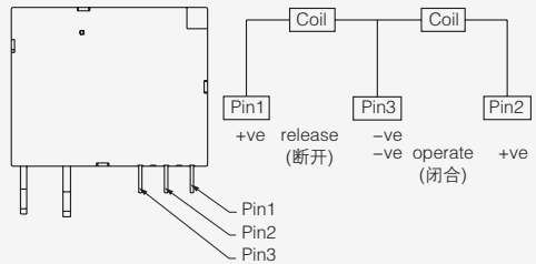
双线圈 Double Coil
